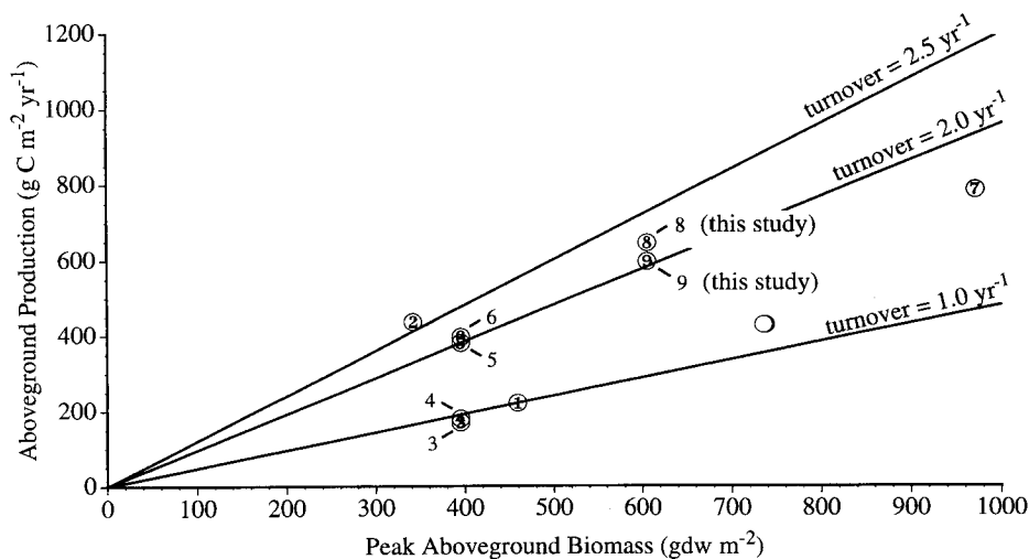
Fig. 8. Aboveground production versus peak biomass for Peltandra virginica and/or Pontederia cordata only in tidal freshwater marshes. Symbols as follows: \circ Whigham et al. (1978); \textcircled{1} Doumlele (1981); \textcircled{2} Pickett (1984); \textcircled{3} Wohlgemuth's (1988) peak biomass, \textcircled{4} Smalley, \textcircled{5} mortality, and \textcircled{6} Allen curve methods; \textcircled{7} Booth (1989); \textcircled{8} this study's peak biomass, and \textcircled{9} Smalley methods. Lines indicate turnover (production/peak biomass) of 1, 2, and 2.5 \text{ yr}^{-1} .
